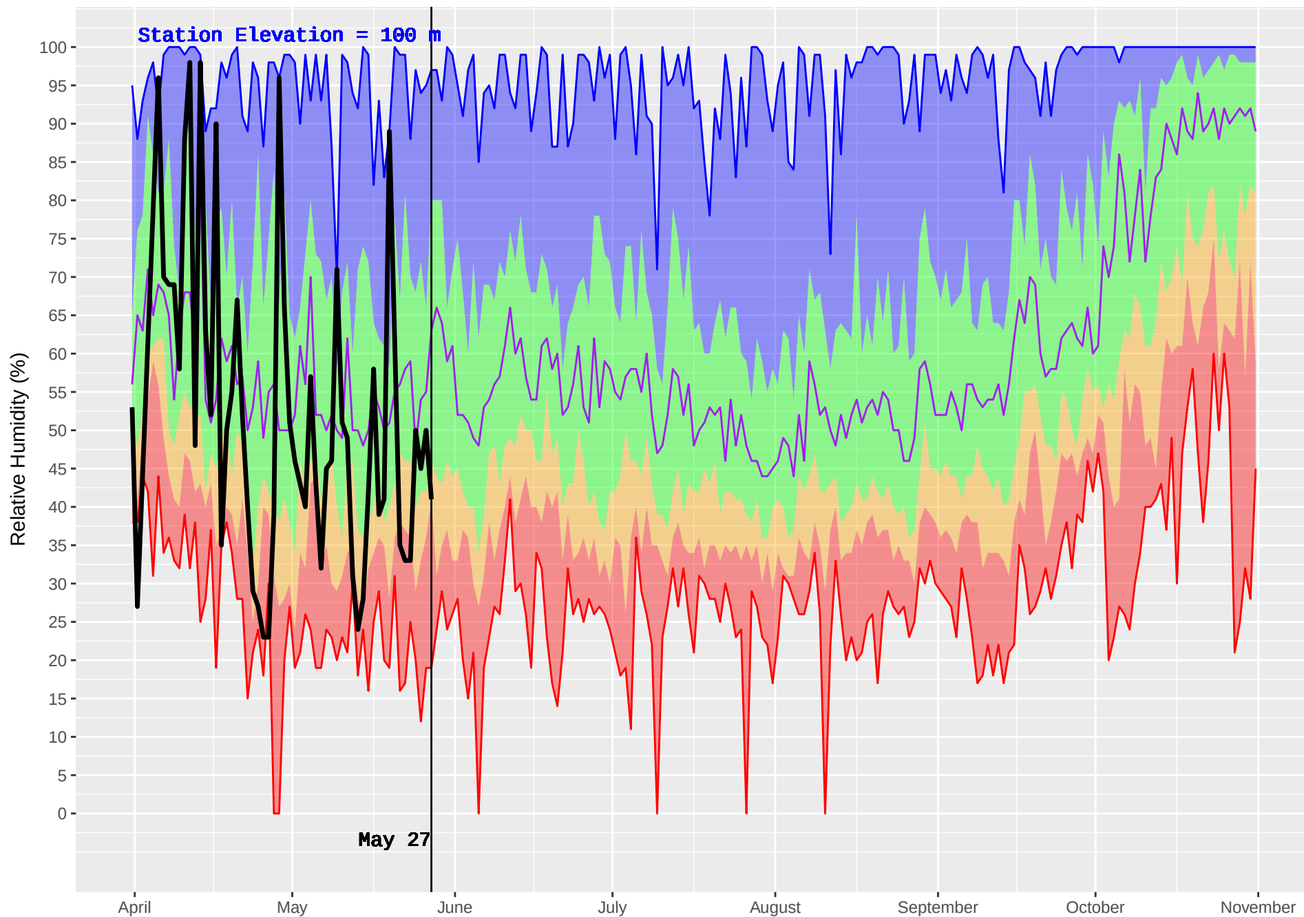
BEAVER CREEK (37) : Historical (1987–2016) and Current (2018) Noon Relative Humidity
