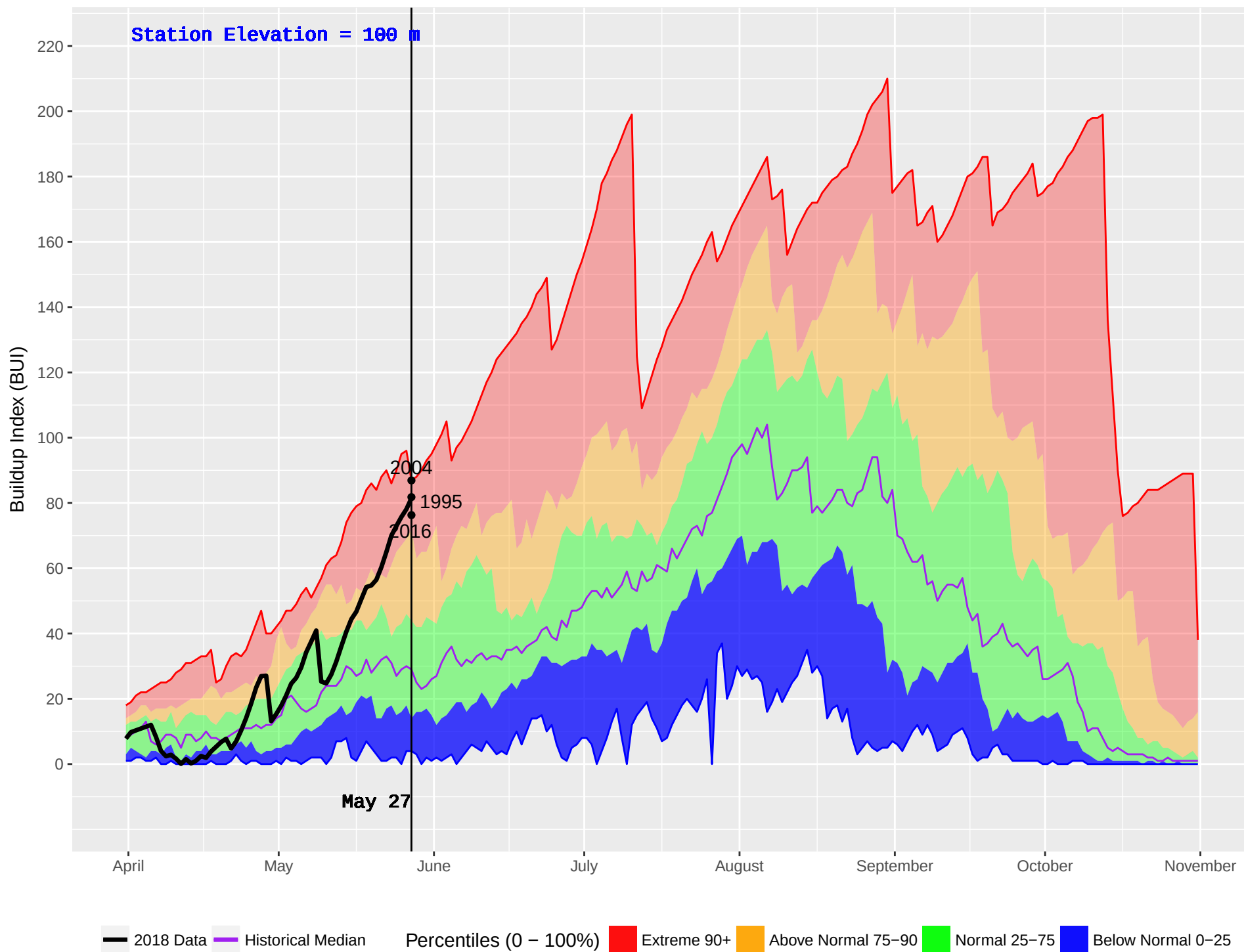
BEAVER CREEK (37) : Historical (1987–2016) and Current (2018) Noon Buildup Index (BUI)
