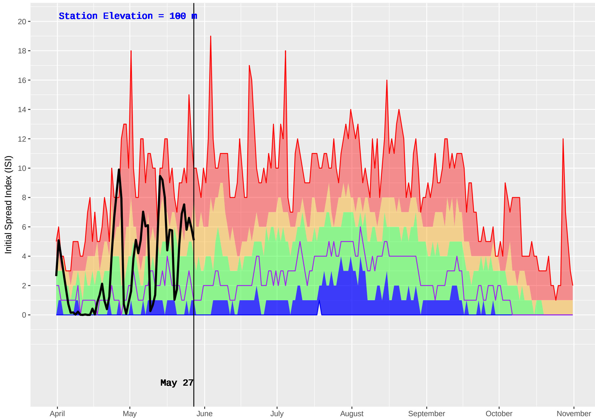
BEAVER CREEK (37) : Historical (1987–2016) and Current (2018) Noon Initial Spread Index (ISI)
